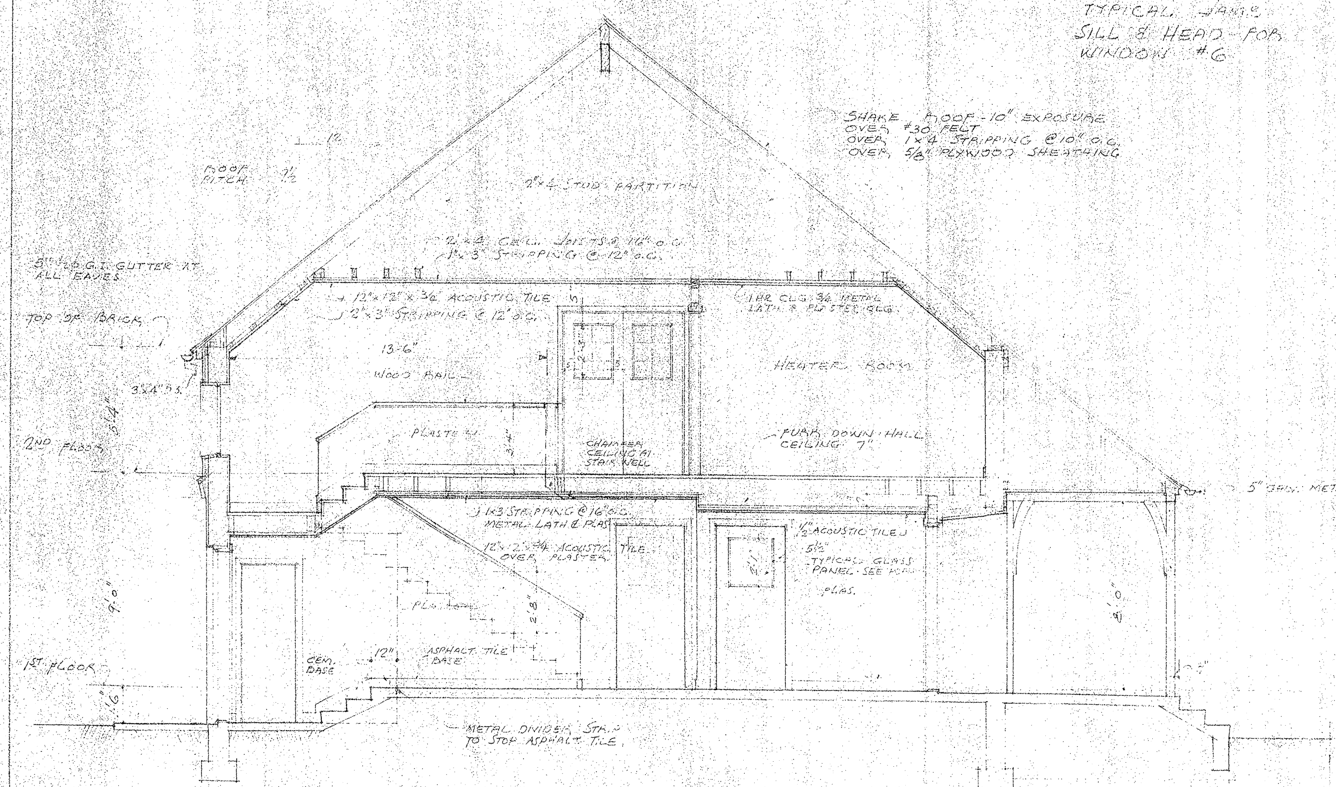
SECTION A SCALE 1/4"=1'-0"
