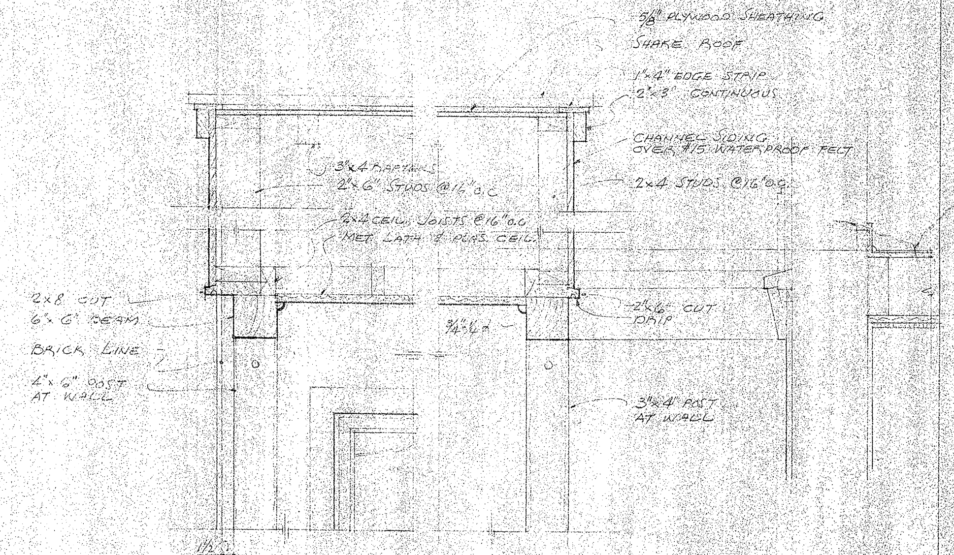
CROSS SECTION PORCH DETAILS (MAIN ENTRANCE) SCALE 1"=1'-0"
