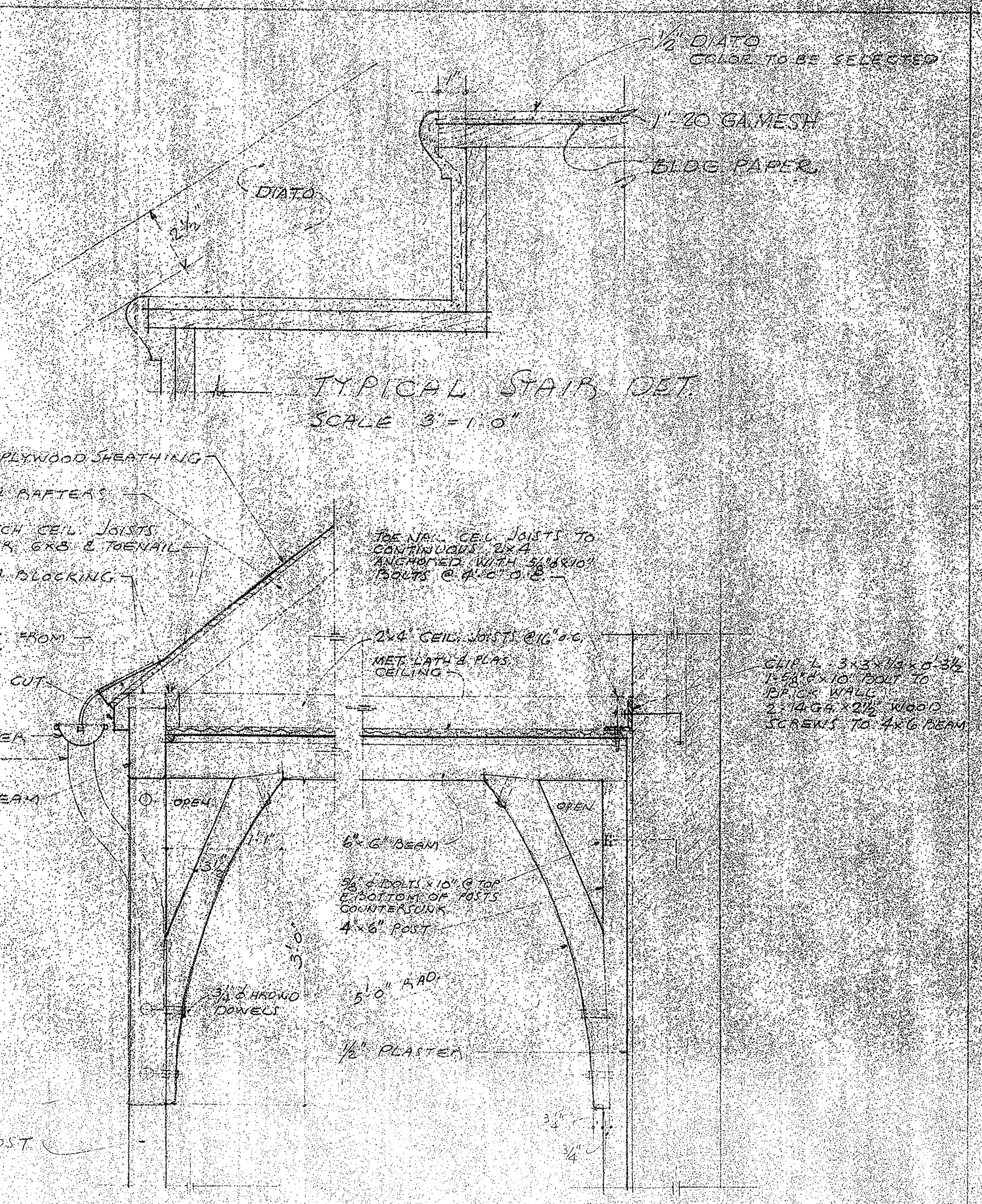
EAVE SECTION
